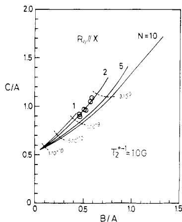
Figure 6. Comparison of experimental (○) and calculated (—) C/A vs. B/A dependence.
