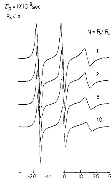
Figure 5. Theoretical spectra of anisotropic rotation about its X axis illustrating the change in the line shape as a function of degree of anisotropy, N . The spectra were calculated for the Brownian diffusion model using a constant rotational correlation time, \tau_R = 1 \times 10^{-9} \text{ s} , and 1/T_2^0 = 0.5 \text{ G} .
